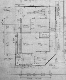
GROUND FLOOR PLAN CUM SITE PLAN.
