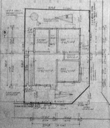
GROUND FLOOR PLAN CUM. SITE PLAN.
